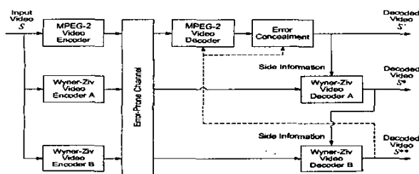
Fig. 1. Wyner-Ziv decoder uses decoded error-concealed video waveform as side information in systematic lossy source-channel setup.
