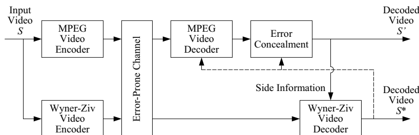
Figure 1. Wyner-Ziv bitstream uses decoded error-concealed video waveform as side information in a systematic lossy source-channel set-up.
