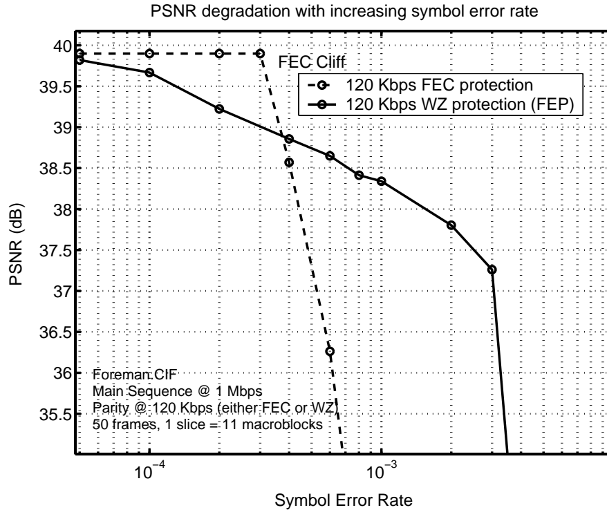
Figure 4. Proposed systematic lossy forward error protection (FEP) scheme outperforms conventional FEC when the symbol error probability increases.
