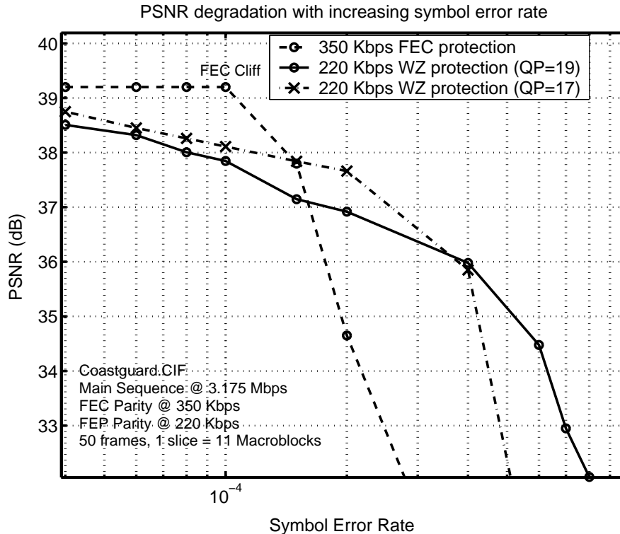
Figure 6. The distortion in the coarse video description can be traded off with the amount of Wyner-Ziv protection to achieve superior overall performance compared to FEC.
