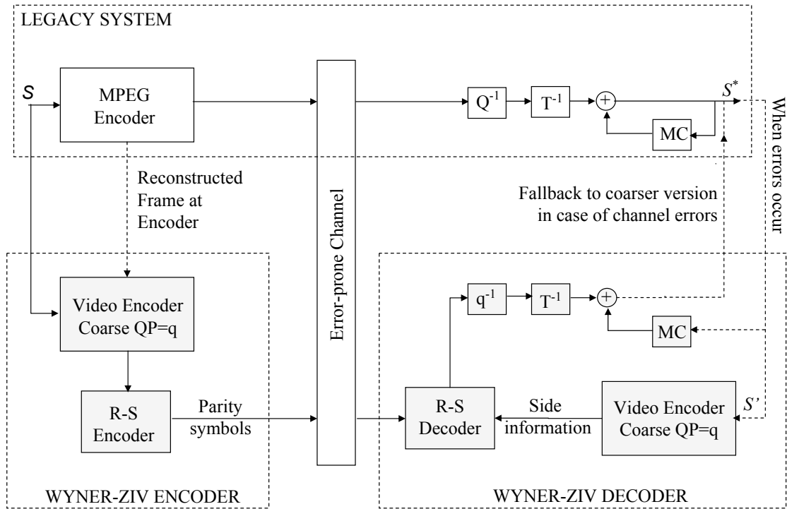
Figure 2. Wyner-Ziv codec in the proposed systematic lossy forward error protection (FEP) scheme
